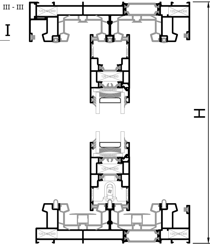
Three Sash Sliding 90 Degrees Cut Right Opening Window with Sash M4544
