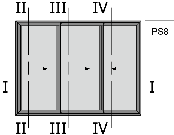
Three Sash Sliding 90 Degrees Cut Right Opening Window with Sash M4544
