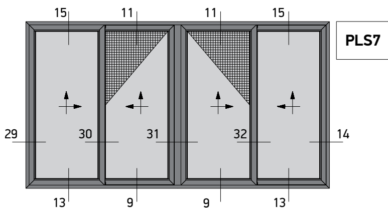
Four Sash Parallel Lift and Slide 45° Cut Right Opening Window with Flyscreen
