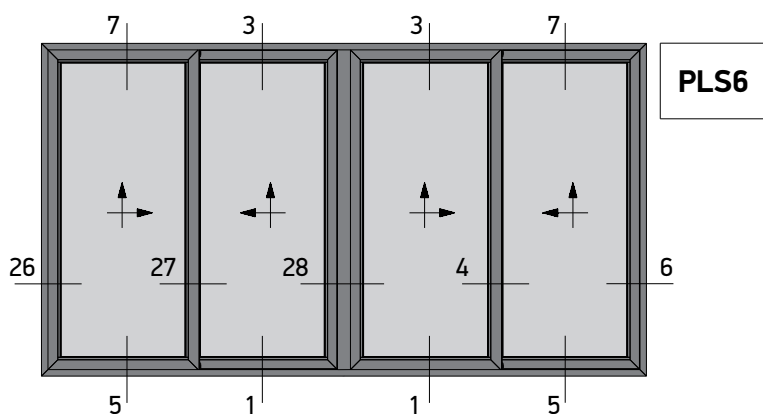
Four Sash Parallel Lift and Slide 45° Cut Right Opening Window
